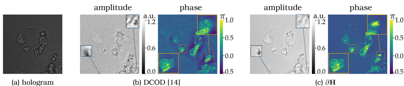
Figure 4. Experiment 3: Verification on a cheek cell sample with the setup in Figure 1c (data from ref. [14]). a) The hologram, b) DCOD, and c) \partial H reconstructions.
