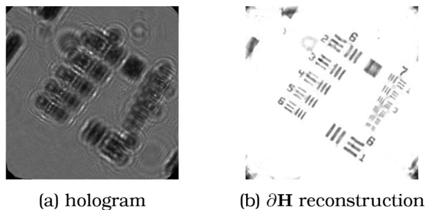
Figure 6. Experiment 5: Intensity-only object imaging with fiber bundle setup of Figure 1d (data from ref. [21]). a) The hologram extracted from a fiber-bundle setup and b) \partial H reconstructions.
