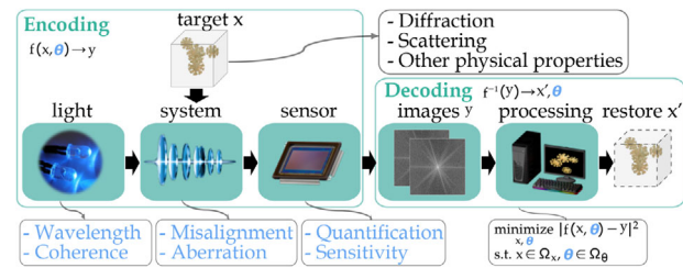
Figure 7. Realistic factors (blue color text represented by \boldsymbol{\theta} ) in a typical holography system that may affect the modeling. \partial H models and retrieves some of these parameters.
