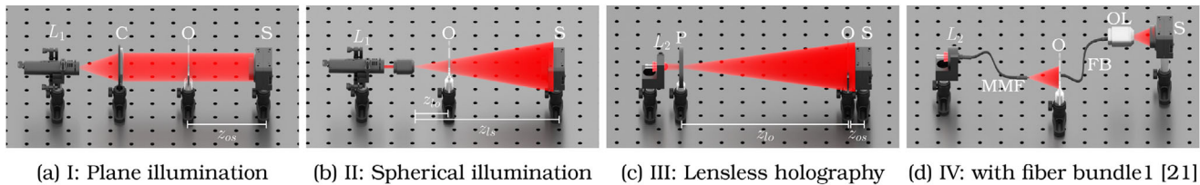
Figure 1. Various inline holography systems that are used for the verification: Inline holography with a) plane wave illumination and b) spherical wave illumination, c) lensless holography and d) lensless holography with fiber bundle setup. L_1 : laser light source; L_2 : LED light source; C: collimator; O: object; P: pinhole; S: camera sensor; MMF: multi-mode fiber; FB: fiber bundle; OL: objective lens.
